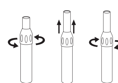
3. Loosen Nut, Extend Pipe Up, Tighten Nut.
